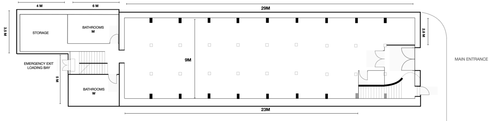
Ground Floor
